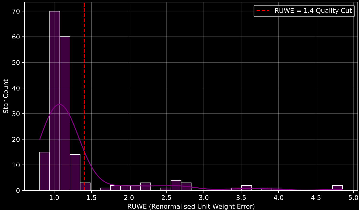
GAPOGEE DR17 Field [002+53_MGA] RUWE Distribution (n= 187)
