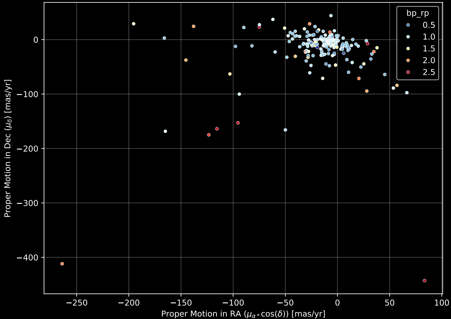
APOGEE DR17 Field: [002+53_MGA] Proper Motion Diagram (n= 197)
